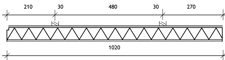
Dwarsdoorsnede sandwich-dakelement
