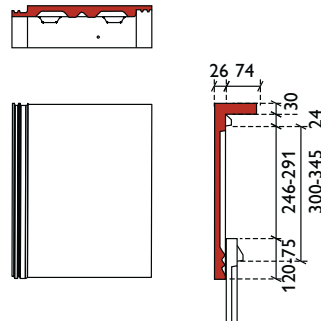
chaperonpan 90°
