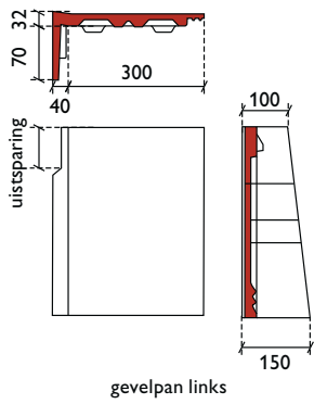
gevelpan links
