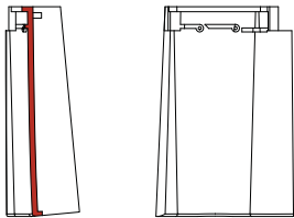
ondergevelpan links
