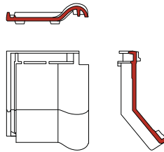
knikpan 140°
