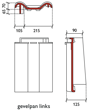
gevelpan links
