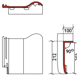
chaperonpan
